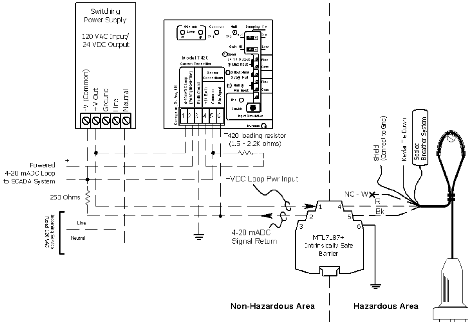
SLX 100-MIS Submersible Level Transducer with a T420 providing a 2 nd 4-20 mA output. The SLX may be powered by a Station Master controller, providing a 4-20 mA input to the Station Master, while the T420 senses the signal and provides a separate (scalable) 4-20 mA output to power another loop. The SLX 130-M is applied in a similar manner
