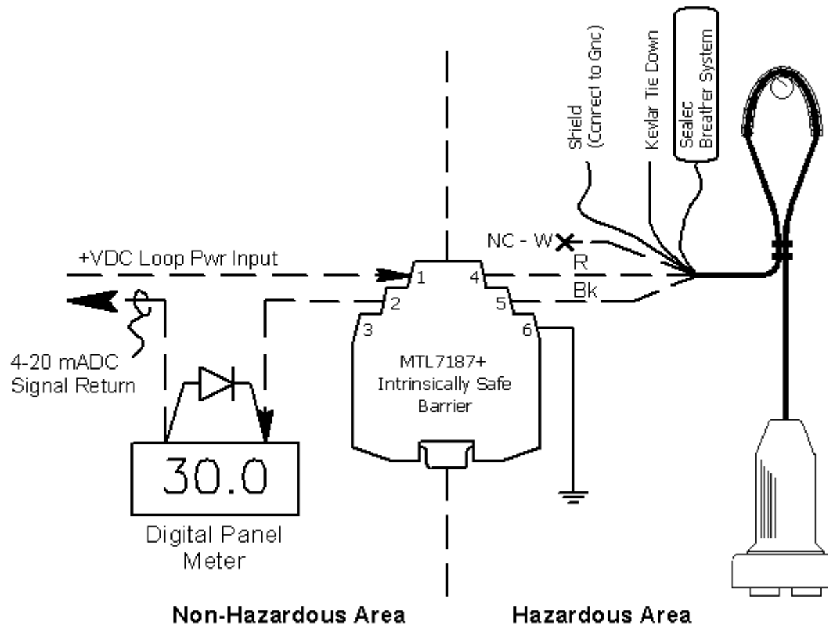
SLX 100-MIS Submersible Level Transducer with a MTL 7187+ Intrinsic Safe Zenner Barrier with a panel meter for local level indication.
