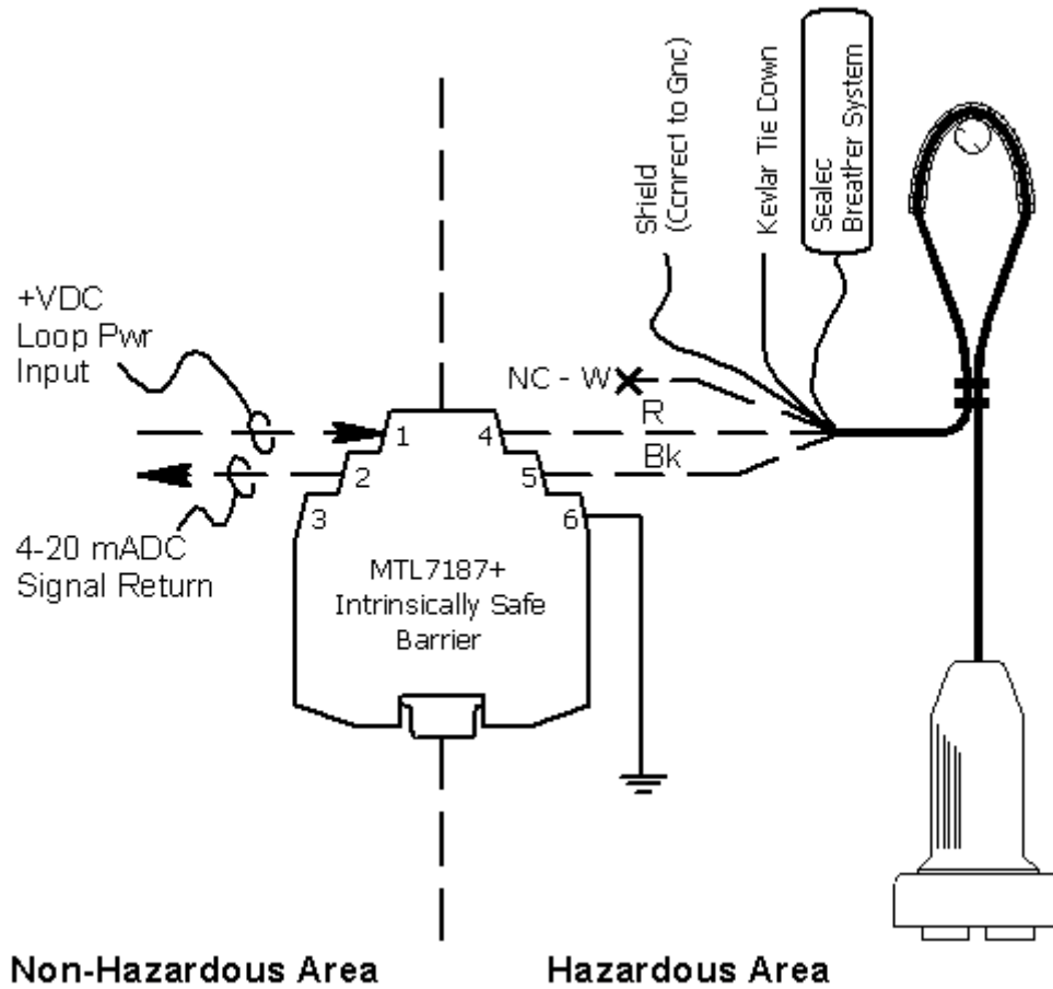
SLX 100-MIS Submersible Level Transducer with a MTL 7187+ Intrinsically Safe Zenner Barrier The SLX 130-MIS is applied in a similar manner
